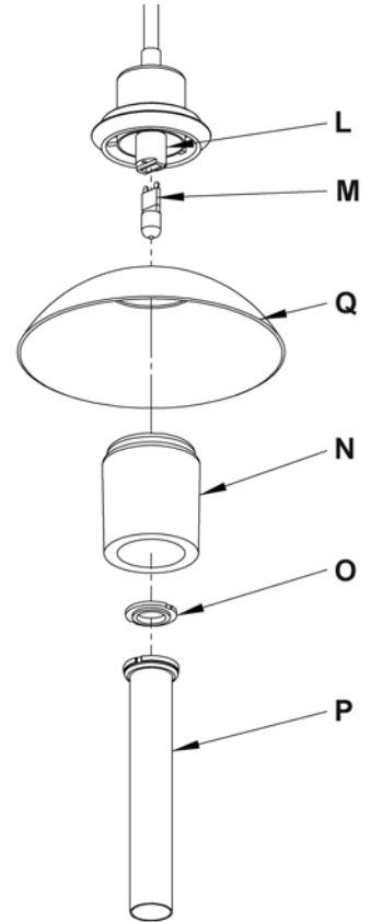
(Figure 5)
